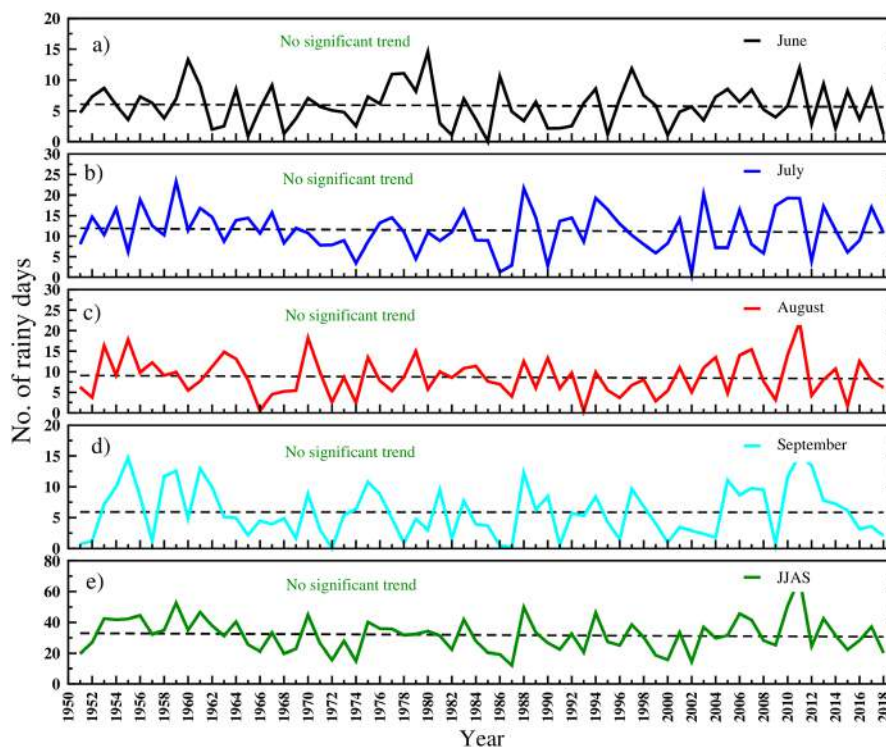
Figure 11: Inter annual variability of rainy days (number of days) over Rajkot for 1951-2018
